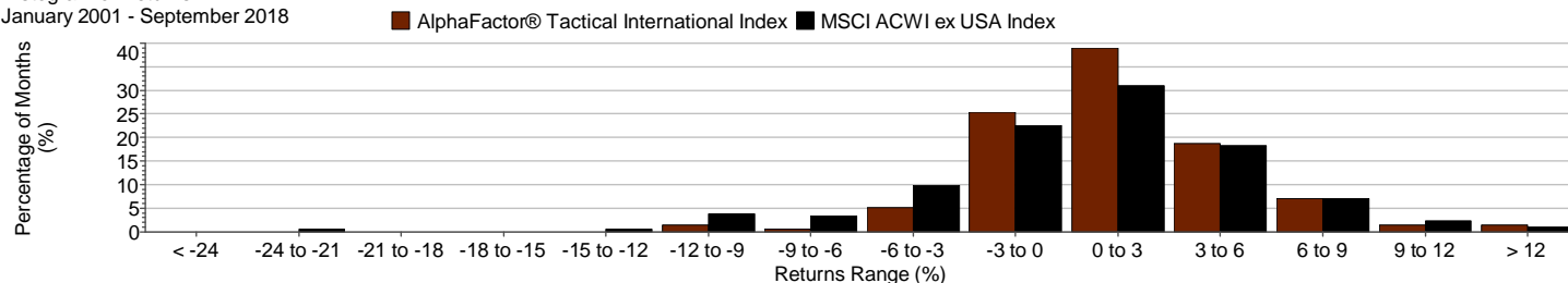
Histogram of Returns January 2001 - September 2018
